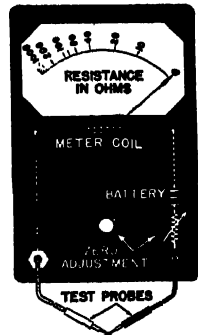
Basic circuit of a series-type ohmmeter.
